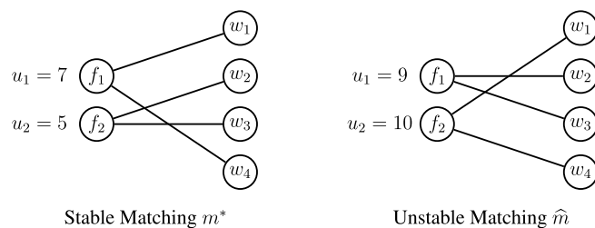
FIGURE 8. Stage-Game Matchings.
