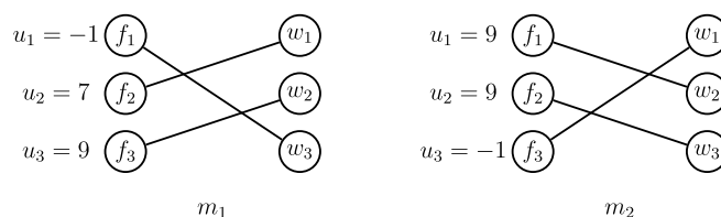
FIGURE 7. Unstable matchings.
