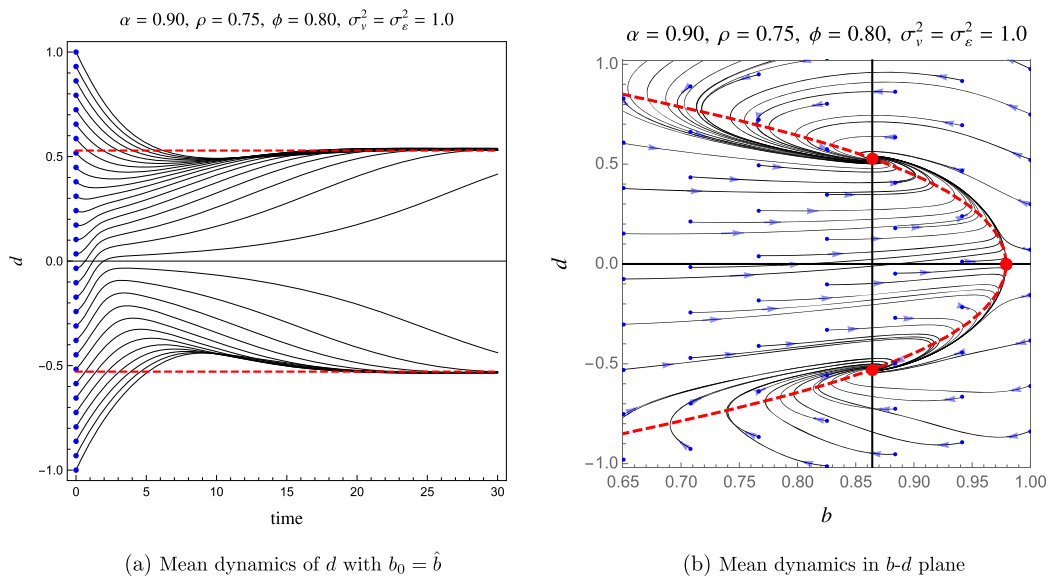
FIGURE 4. Mean dynamics.
