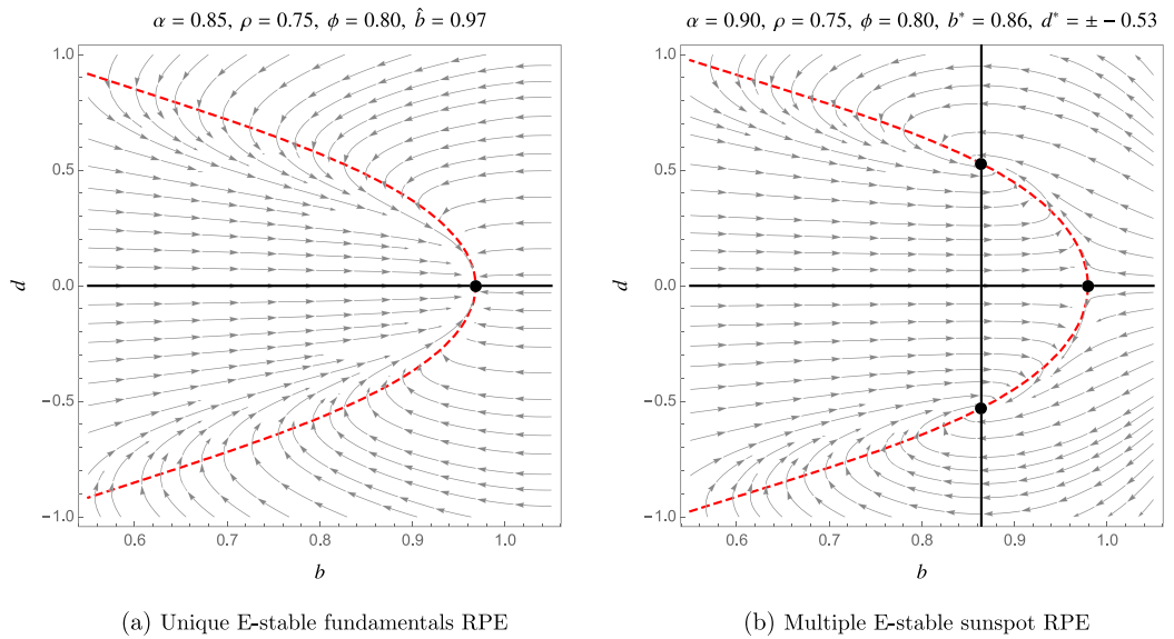
FIGURE 2. E-stability dynamics.
