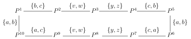
FIGURE 5. The environment \tilde{G} = \langle \tilde{\mathcal{D}}, \mathcal{E}^{\text{adj}} \rangle .
