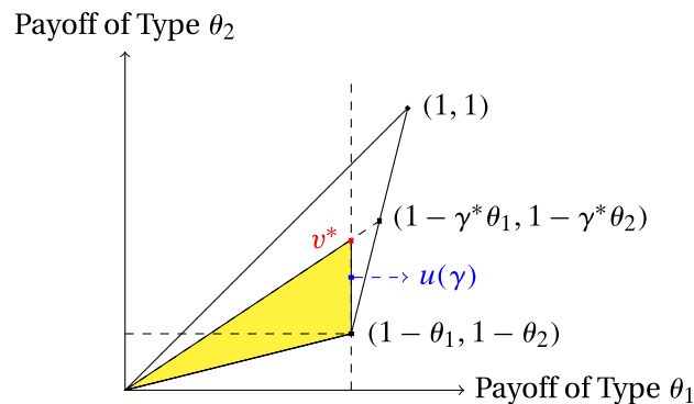
FIGURE 2. Player 1's highest equilibrium payoff v^* , her equilibrium payoff set (shaded area), and payoff u(\gamma) for some \gamma \in (\gamma^*, 1) .
