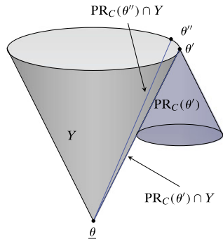
FIGURE 7. The cone of the biases C has infinitely many extreme rays. There is no local punishment for the deviation (\theta', \theta'') , even though there exists a global punishment \underline{\theta} .
