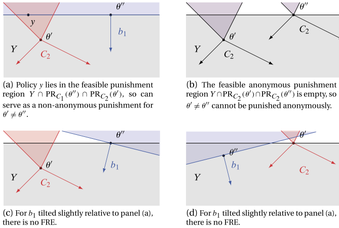
FIGURE 6. Non-anonymous vs. anonymous FRE.
