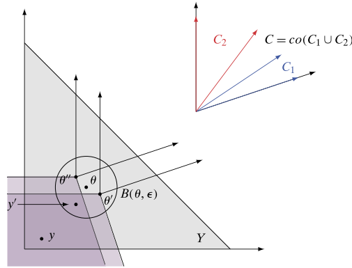
FIGURE 2. The dark shaded area is the feasible anonymous punishment region: Y \cap \text{PR}_C(\theta') \cap \text{PR}_C(\theta'') . Whenever an anonymous punishment is feasible, a robust anonymous punishment is feasible.
