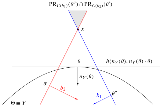
FIGURE 10. If there is no FRE, then the LDC is violated.
