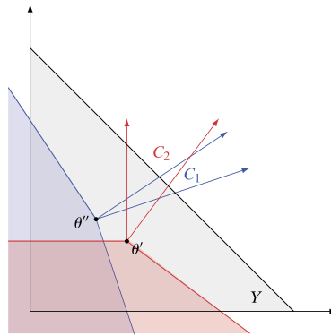
FIGURE 1. The shaded areas with vertices \theta'' and \theta' represent \text{PR}_{C_1}(\theta'') and \text{PR}_{C_2}(\theta') , respectively. The joint intersection of these areas with the policy space Y is the feasible punishment region for the incompatible reports \theta', \theta'' , given supports C_1, C_2 .
