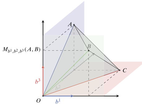
FIGURE 9. There exists an anonymous FRE given C(b^1, b^2, b^3) but M_{b^1, b^2, b^3}(A, B) \cap Y = \emptyset .
