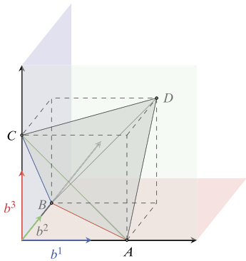
FIGURE 8. There is no FRE given C(b^1, b^2, b^3) , but for any pair of extreme biases b^i, b^j , there exists a FRE given C(b^i) and C(b^j) .
