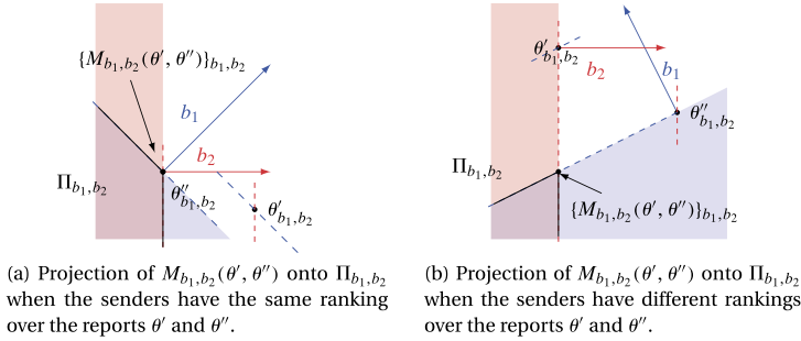
FIGURE 4. Projection of M_{b_1, b_2}(\theta', \theta'') onto \Pi_{b_1, b_2} .
