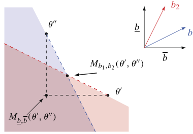
FIGURE 5. The uncertain biases have support C(\underline{b}, \bar{b}) . For any realization b_1, b_2 \in C(\underline{b}, \bar{b}) , M_{\underline{b}, \bar{b}}(\theta', \theta'') is an anonymous punishment.
