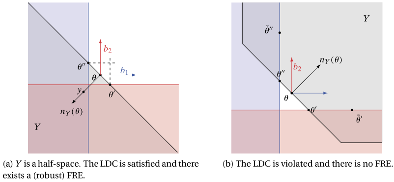
FIGURE 3. The LDC for Y \subset \mathbb{R}^2 .
